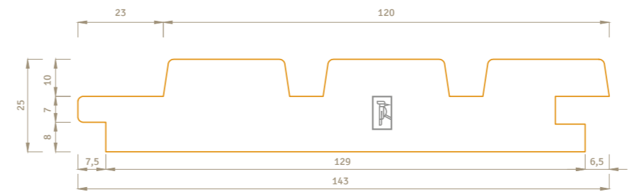
TRIPLE RHOMBUS
