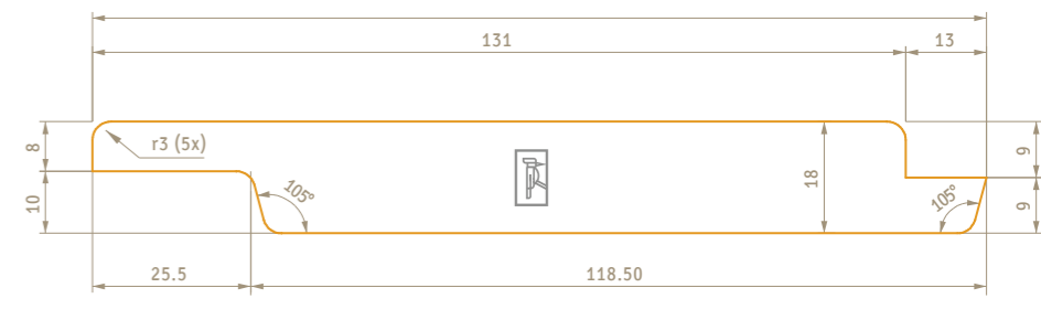
CHANNELSIDING
