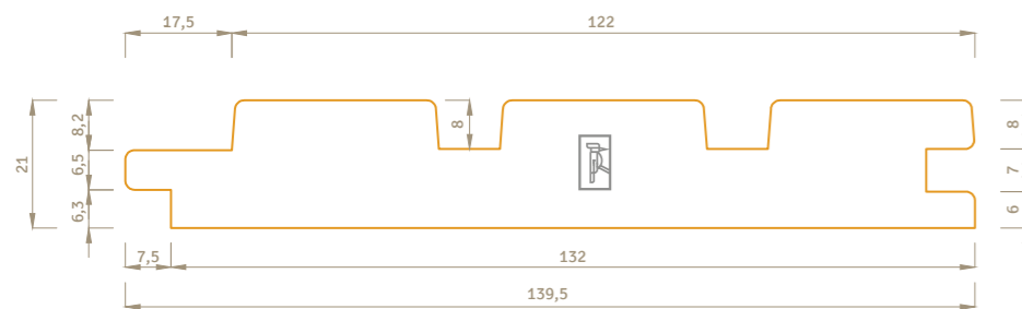
TRIPLE RHOMBUS
